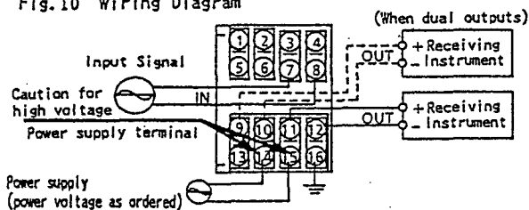
Fig.10 Wiring Diagram
