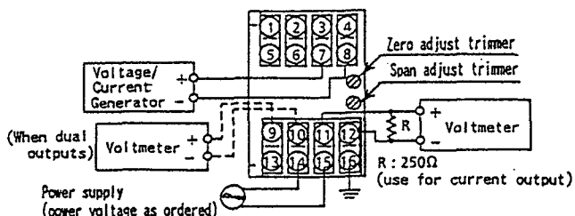
Fig.11 Wiring of Calibration Equipment
