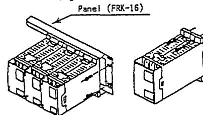
Fig.2 Wall Mounting
